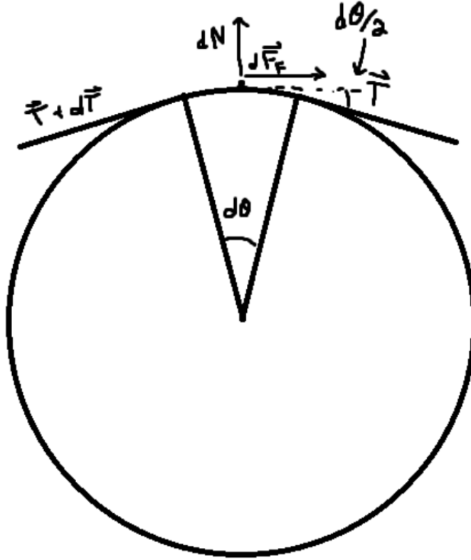
Figure 25: Free-body diagram of a differential belt element spanning d\theta .
